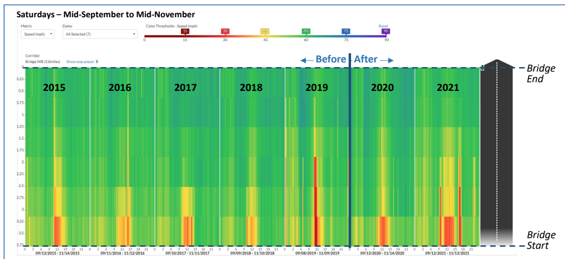
Figure 8-61: Speed Maps – I-580 West – Bridge – Saturdays, Fall 2015-2021
