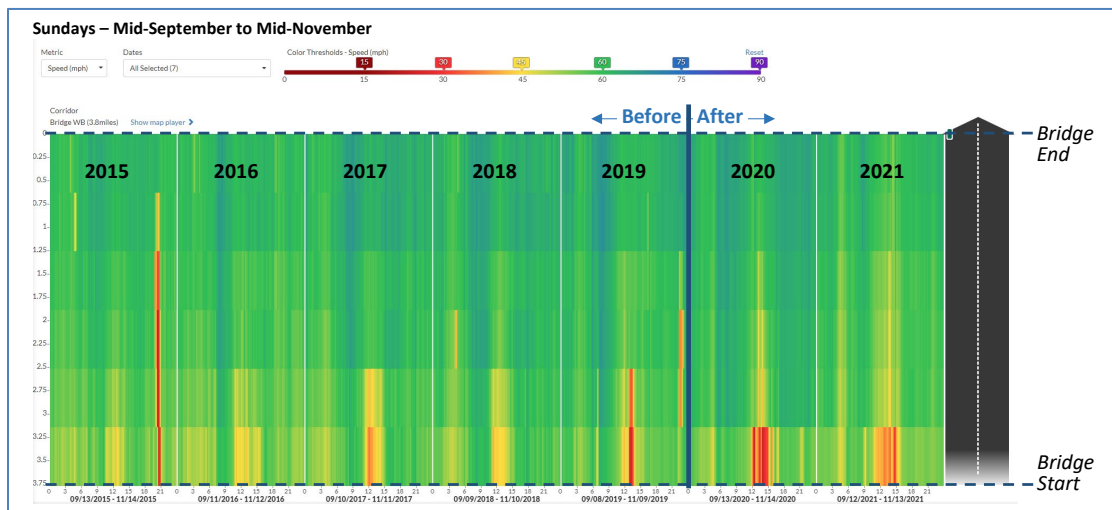
Figure 8-62: Speed Maps – I-580 West – Bridge – Sundays, Fall 2015-2021
