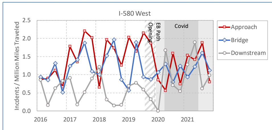
Figure 10-8: Number of Accidents by Quarter – I-580 West, 2016-2021
